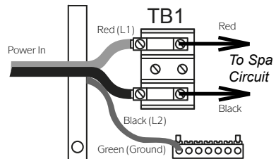
Illustration 4: 3-Wire/240 VAC Connection for J-230/J-270/J-280/J-325/J-335/ J-345/J-355/J-365/J-460/J-465/J-470/ J-480 models.
