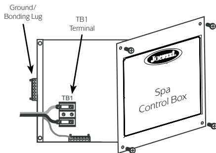
Illustration 3: Control Box
