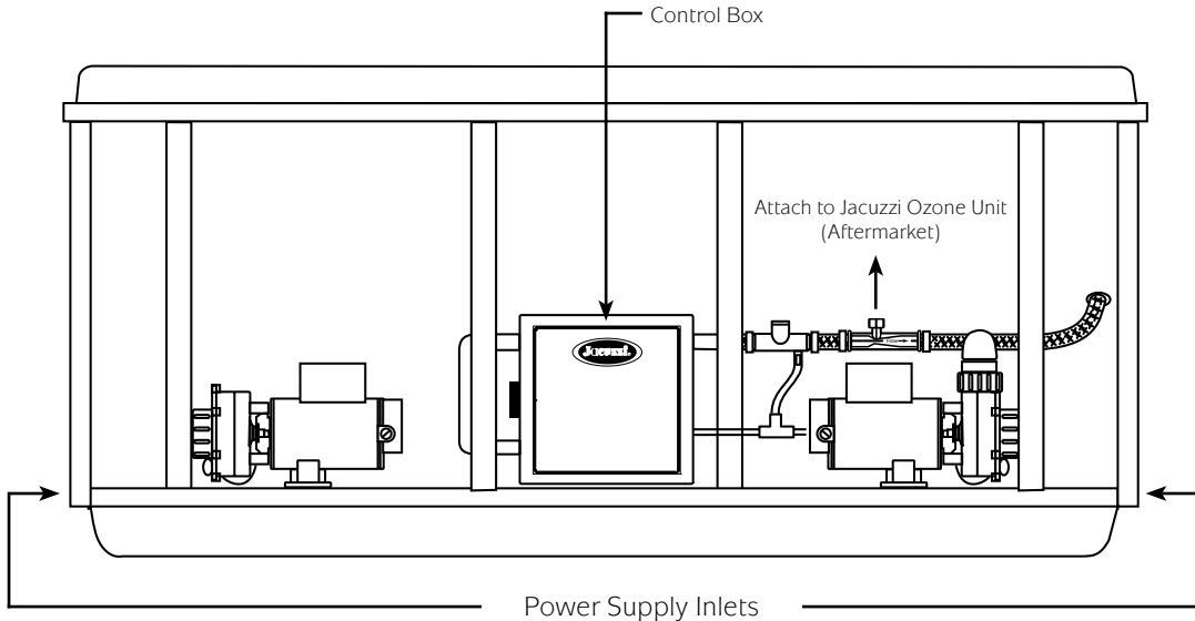
Illustration 2: The spa's equipment compartment.
