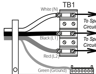
Illustration 8: 4-Wire/240 VAC Connection for J-210/J-220/J-315 models. (Hard Wired Connections Only)
