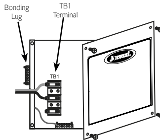
Illustration 6: Control Box for J-210/J-220/J-315 models.
