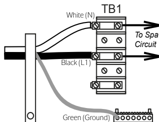
Illustration 7: 3-Wire/120 VAC Connection for J-210/J-220/J-315 models. (Supplied GFCI Cord or Hard Wired 3-Wire Connection)
